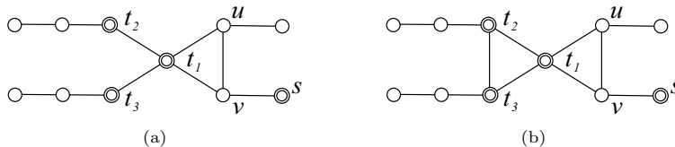
Fig. 4: Examples of hard-to-handle cases. Removing any edge of the triangle \langle t_1, u, v \rangle in each graph results in violating the conditions C1 and C2 , respectively.
