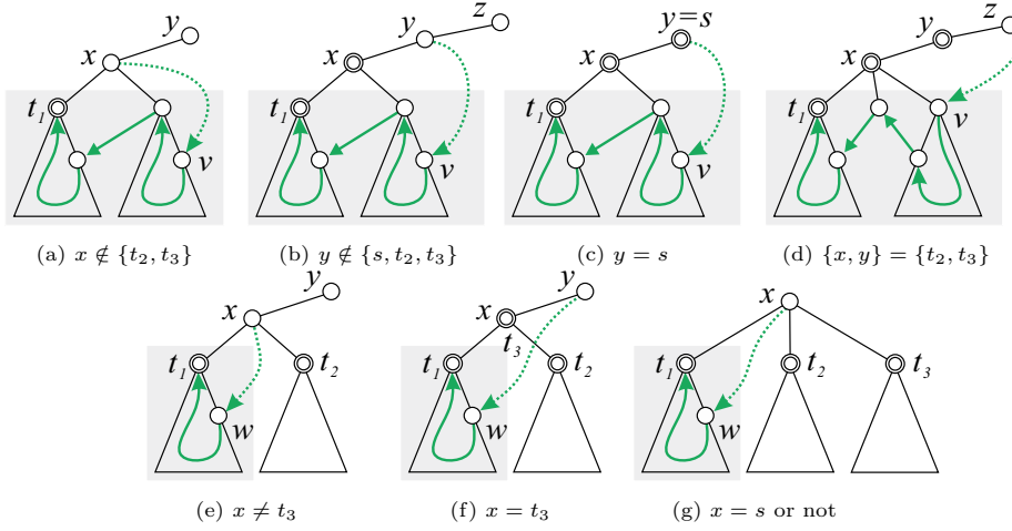
Fig. 2: Hybrid subcases in the description of Algorithm 2: (a) to (d) for \text{numSinks}[x] = 1 , (e) and (f) for \text{numSinks}[x] = 2 , and (g) for \text{numSinks}[x] = 3 .
