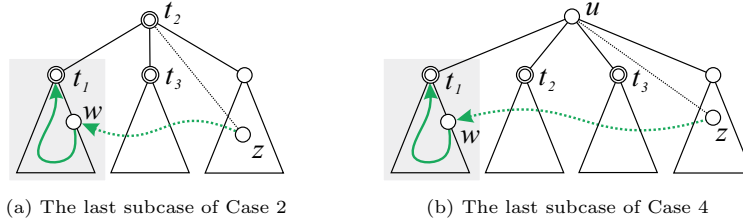
Fig. 3: Two hybrid subcases in the proof of Theorem 5.
